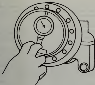
FIGURE 10-1. Checking cylinder bore with a dial indicator.
